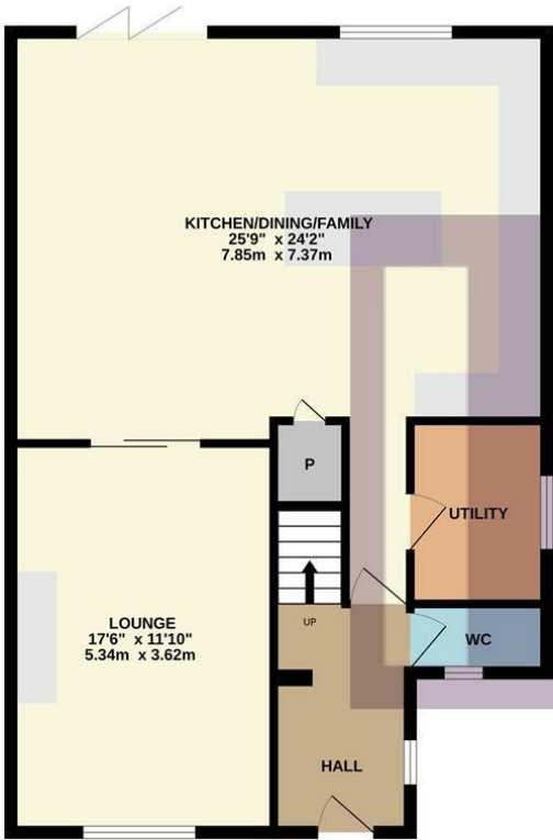
GROUND FLOOR 826 sq.ft. (76.7 sq.m.) approx.
